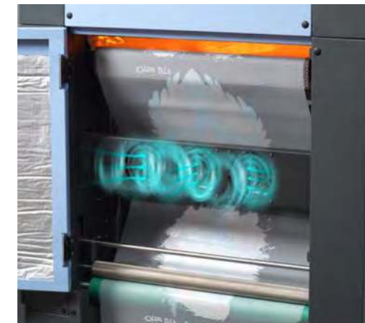
Built-in Fans After the printed film is baked in the oven, the built-in fans accelerate film cooling and improve work efficiency.
